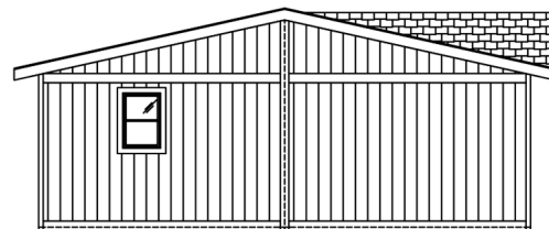
REAR ENDWALL
